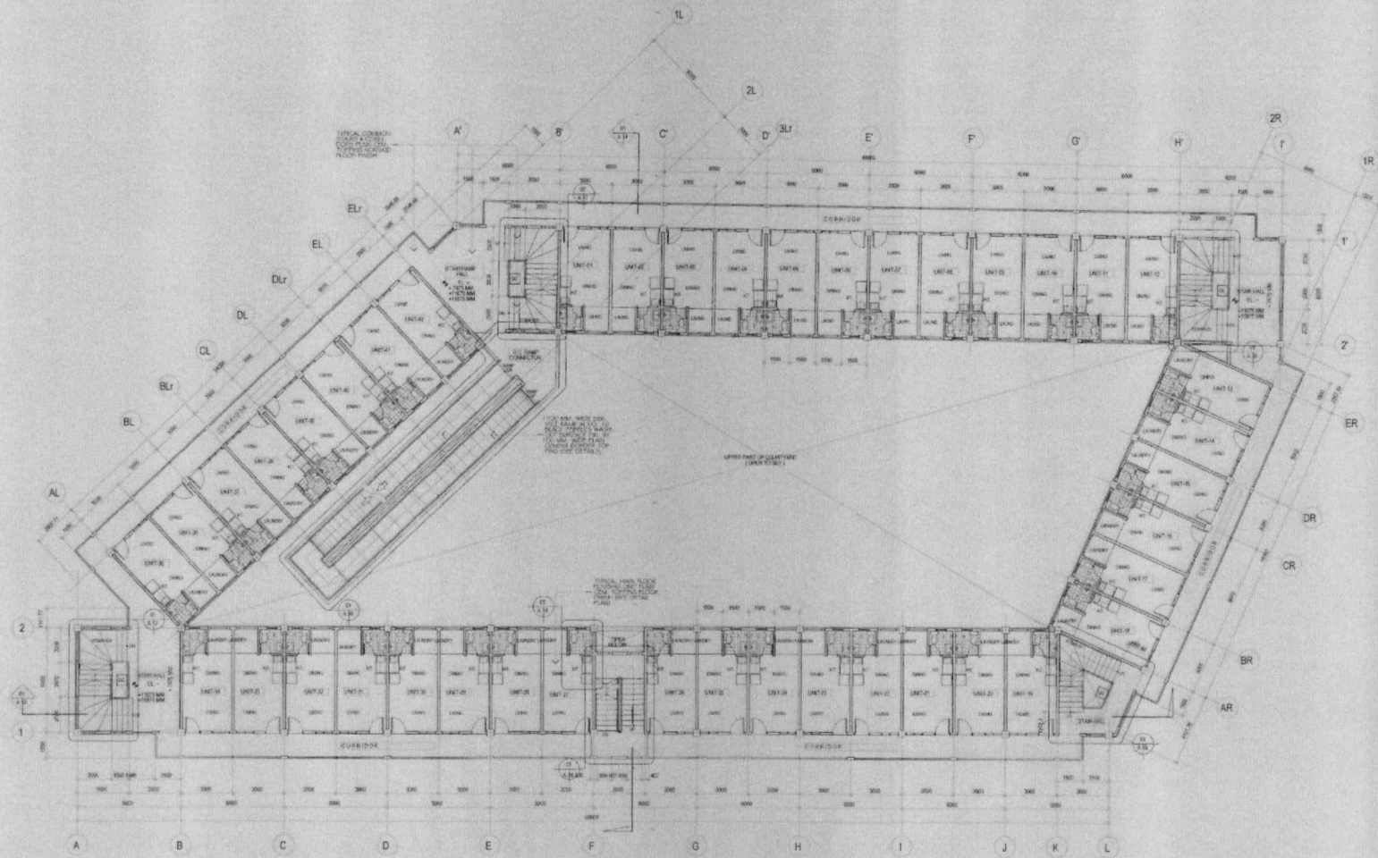
SIERRA MADRE BLDG TYPICAL 2ND TO 4TH FLOOR PLAN
